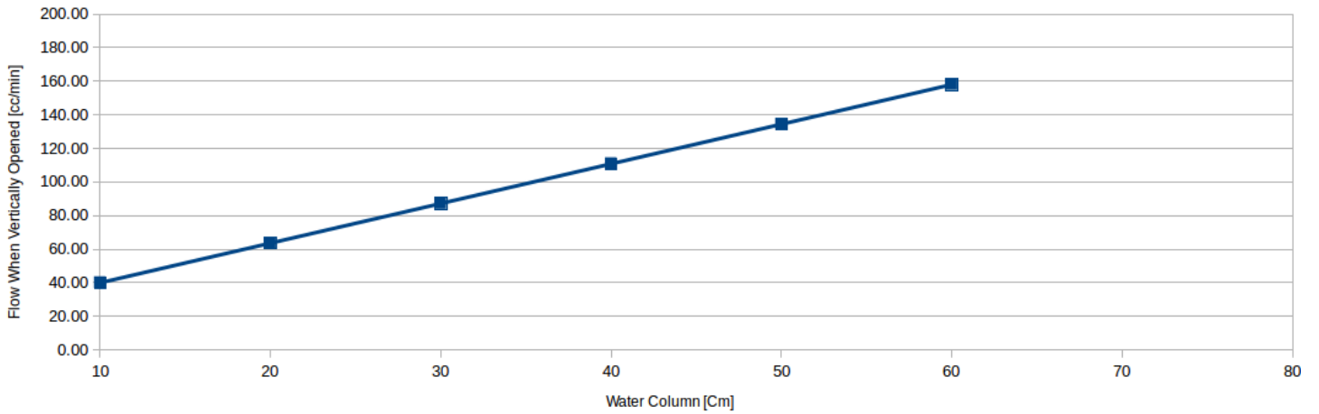
Water flow for 4002H +- 15%
