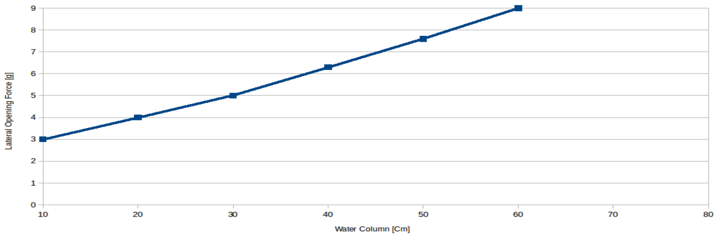
Opening forces for 4002 H +- 15%
