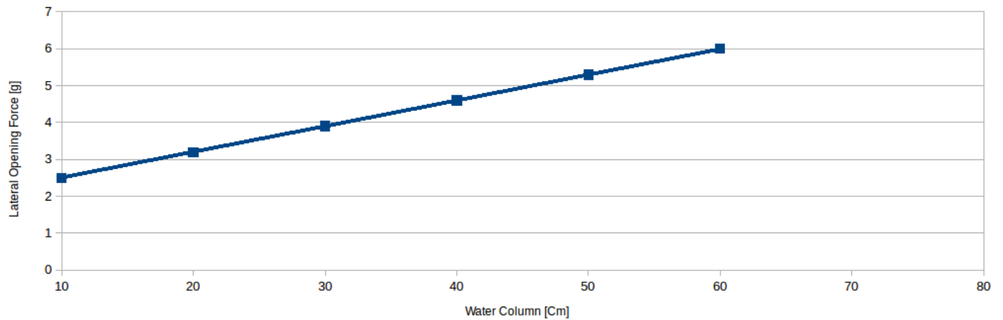
Opening forces for 4006HH +- 15%
