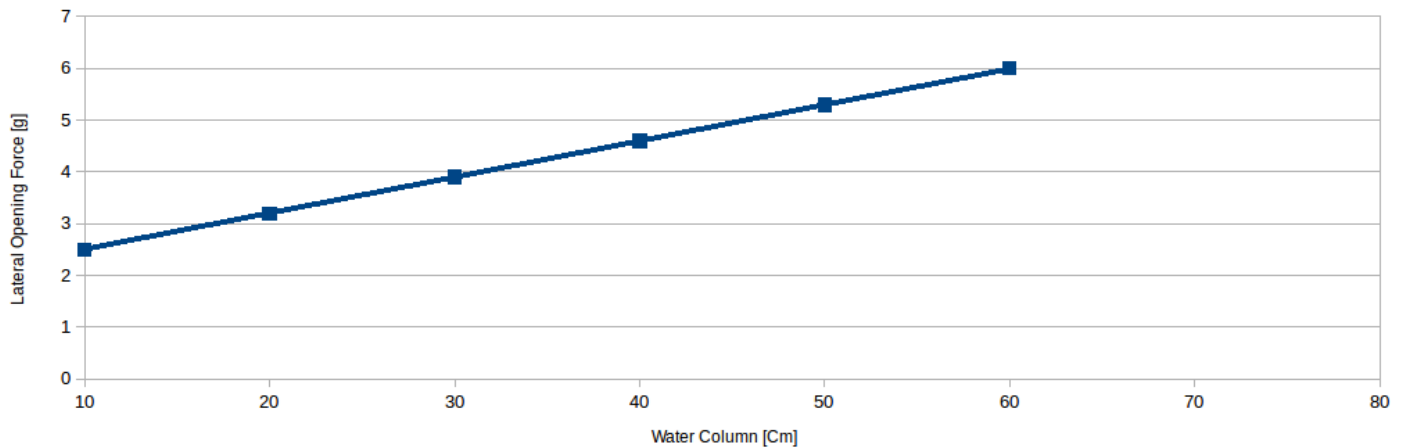
Opening forces for 4006H +- 15%
