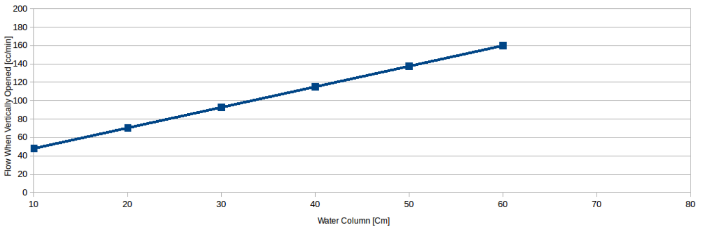
Water flow for 4006H +- 15%
