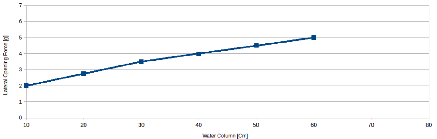
Opening forces for 4006i +- 15%
