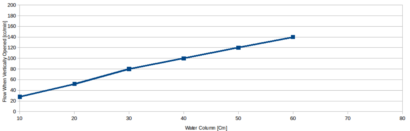
Water flow for 4006i +- 15%
