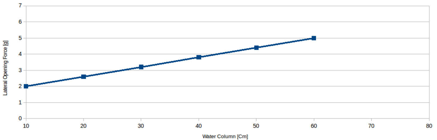
Opening forces for 4007H +- 15%
