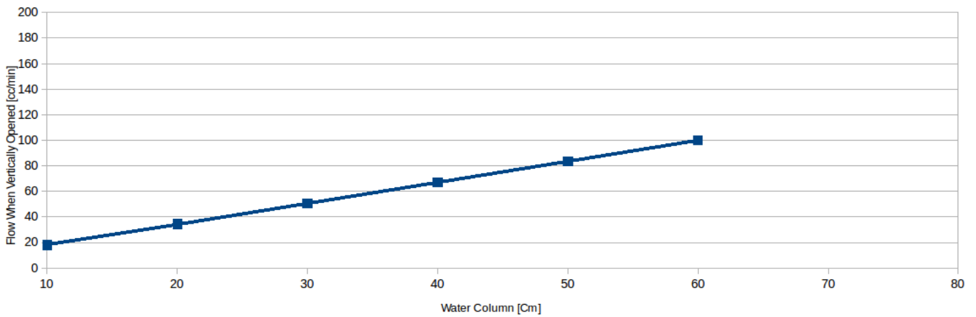
Water flow for 4007H +- 15%
