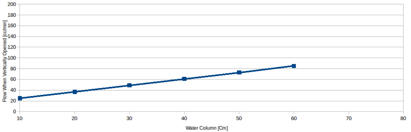
Water flow for 4731G/AQ +/- 15%
