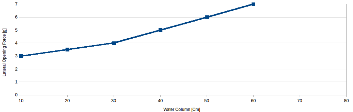
Opening forces for 4731G +/- 15%
