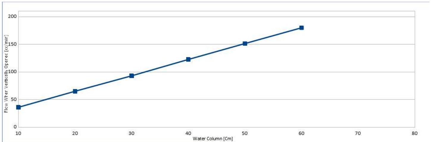
Water flow for 4002HH +- 15%
