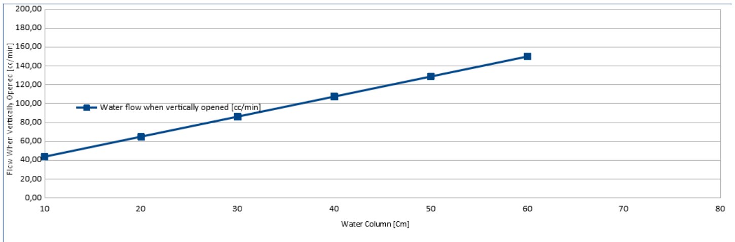
Water flow for 4731HH +- 15%
