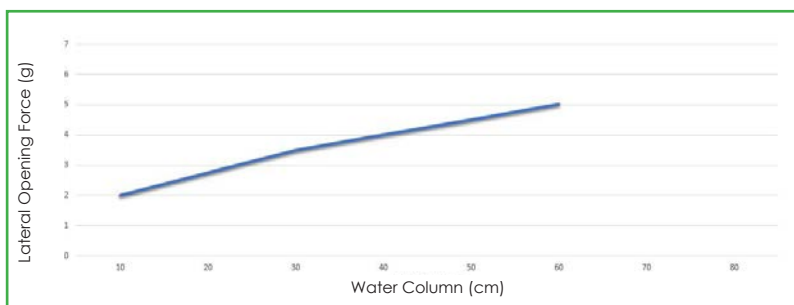
Opening Forces, +-15% Ref. 4006i
