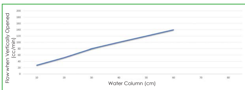
Water Flow, +-15% Ref. 4006i
