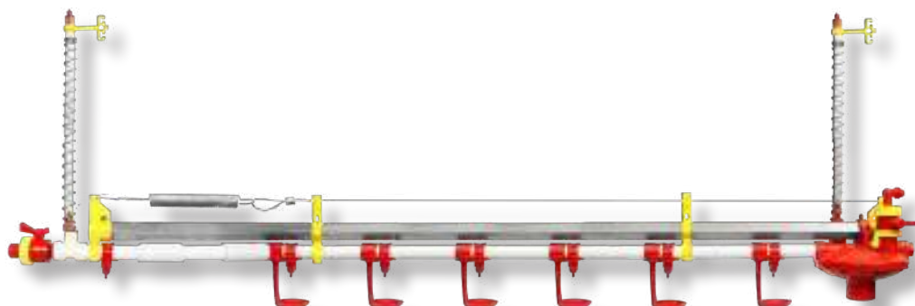
Drinking line with round pipe (ø 26.6 mm)
