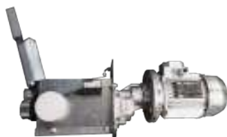
4473T3/4SC Drive unit with three-phase motor 0.75 KW for capacitive sensor
