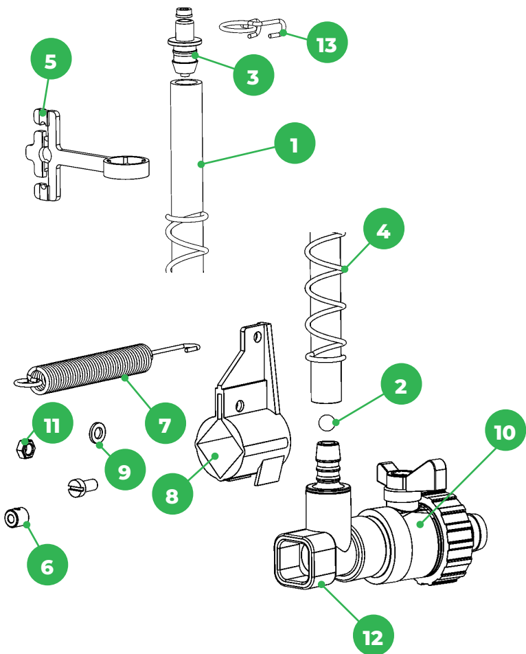
4957N End-of-line kit for square pipe h: 500mm, ø12mm 4957F Flushing version with art.4773 P
