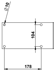
4426 Mounting plate kit for winch 4425
